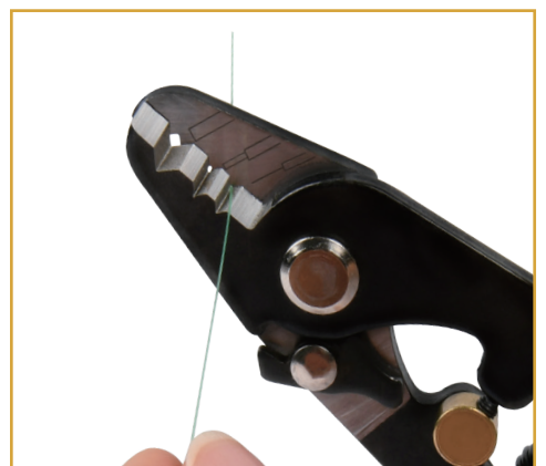
Small hole: strip 250 \mu\text{m} ~125 \mu\text{m} fiber coating
